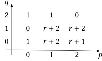
Figure 6.4. Dimensions of E_2 for r = 1, 2
