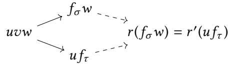
Figure 5.1. A solvable overlap ambiguity
