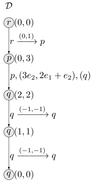
Figure 45: An incrementing derivation tree \mathcal{D} for the 2\text{MVASS}_2 \mathcal{A} = \langle Q, U, M, \preceq \rangle with Q = \{r, p, q\} , U = \{(r, (0, 1), p), (q, (-1, -1), q)\} , M = \{(p, S_1, (q, q)), (p, S_2, (q))\} , and \preceq defined as \{(1, 1), (1, 2), (2, 2)\} . S_1 is the linear set with offset \bar{0} generated by S_0 and B_1 = \{(e_2, e_1, e_1)\} , while S_2 is generated by S_0 and B_2 = \{(e_2, e_1)\} . The first rule of M is not used in this incrementing derivation tree. Notice that we are using twice the incrementing nature of the derivation: once at the beginning with a unary rule and once afterwards for a branching rule.
