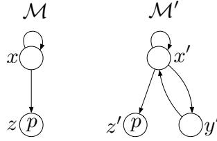
Figure 5: Similarity in both directions does not imply bisimilarity: it is trivial to see that \mathcal{M}, x \Rightarrow \mathcal{M}', x' holds, and it can be seen that \mathcal{M}', x' \Rightarrow \mathcal{M}, x via Z = \{(x', x), (z', z), (y', x)\} ; however, \mathcal{M}, x \not\Leftarrow \mathcal{M}', x' , as any bisimulation Z including (x, x') would need to relate y' to some node w in M , and that would violate Harmony in the case of w = z and Zig in the case of w = x (since from x we can move to z , which satisfies p unlike x' , the only possible neighbor of y' , and as such (z, x') \notin Z ).
