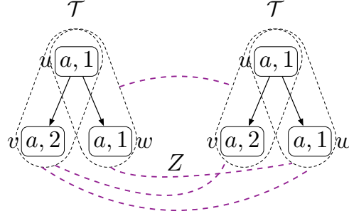
Figure 20: \mathcal{T}, u, w \leftrightarrow^\downarrow \mathcal{T}, u, v , as witnessed by the represented binary XPath = (↓)-bisimulation Z between the same data tree \mathcal{T} . Pairs (u, u)Z(u, u) , (v, v)Z(v, v) , (w, w)Z(w, w) , (w, w)Z(v, v) and (v, v)Z(w, w) are not shown.
