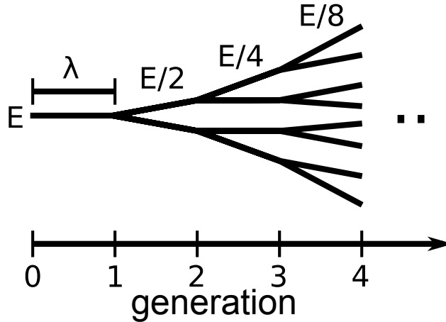
Figure 2.3 Heitler model for the evolution of an atmospheric shower. The interaction length \lambda defines the distance between generations. In each generation the number of particles is multiplied.
