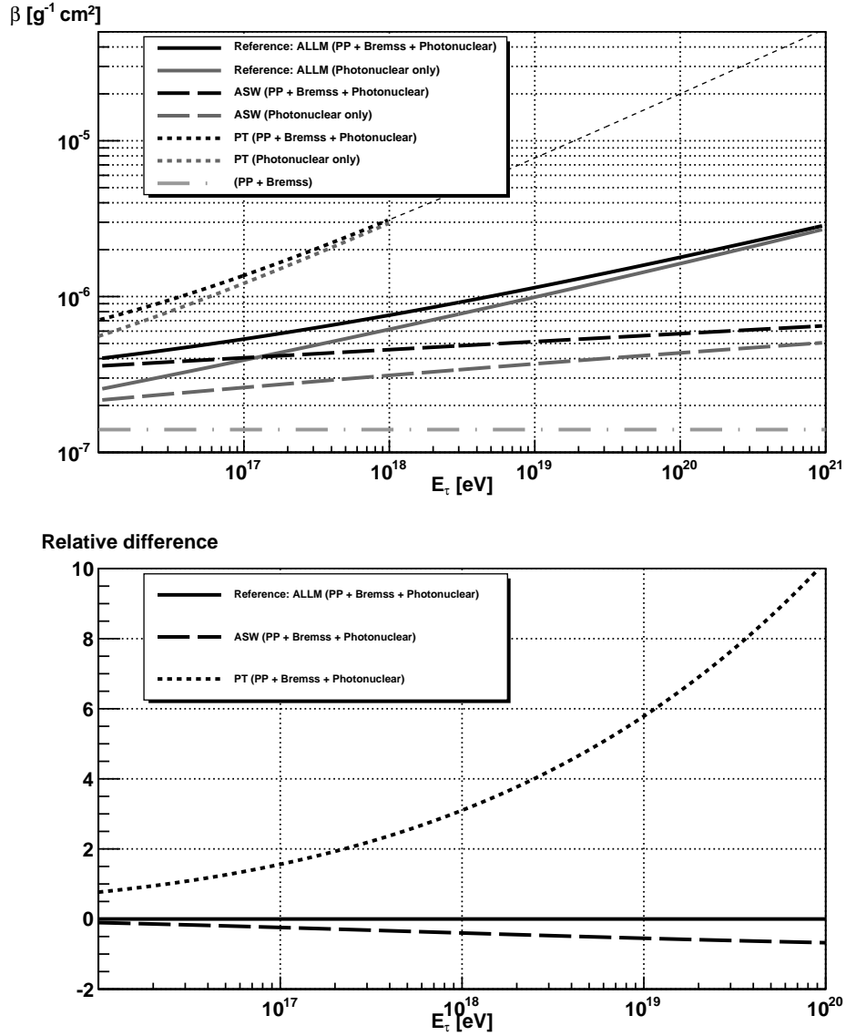
Figure 4.3 Top panel: Tau energy losses in standard rock ( A=22 ). In grey dot-dashed the contribution from pair-production (PP) and bremsstrahlung (Brems) dominated by PP (see text for details). In (dashed/dotted) grey solid the contribution from photonuclear effect for the ALLM (ASW/PT) parametrization. In black the sum of the three processes. Bottom panel: The relative difference between ASW (PT) and the reference model, ALLM.
