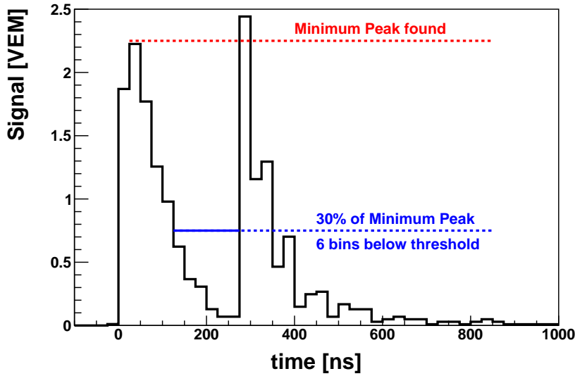
Figure 6.11 Calibrated signal of the event 2629688, station 882 and PMT 1. Two clear peaks are present with 6 contiguous bins below threshold in between.
