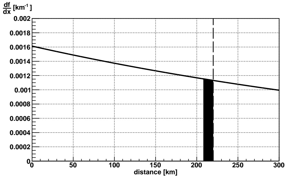
Figure 4.5 Interaction probability density of a 10^{18} eV neutrino skimming the Earth at 1^\circ below the horizon. At this angle the distance that a neutrino has to go through is 220 km. The surface of the Earth is marked with a dashed line. The differential probability is an exponential with \lambda_{int} = 620 km. The approximate depths where on average an interacting neutrino can give rise to an emerging \tau is shown with the black area, and corresponds to 1.4% of the incident flux.
