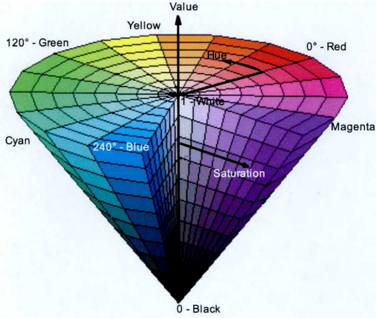
Fig. 2.6: HSV Color Space.
