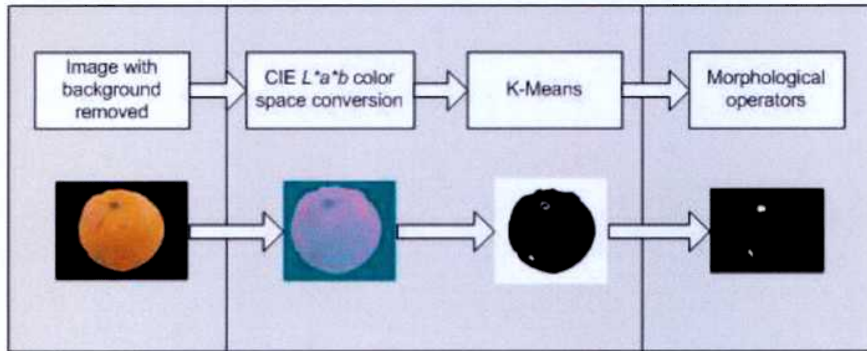
Fig. 4.6: K-Means clustering after performing CIE L^*a^*b colorspace conversion
