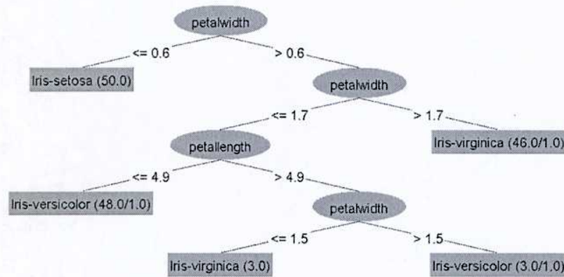
Fig. 2.12: J48 Decision tree for the Iris dataset
