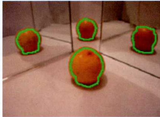
Fig. 4.5: Mirror segmentation
