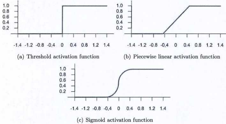
Fig. 2.15: Activation functions
