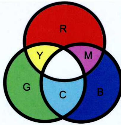
Fig. 2.2: Additive Colors of light: Adding Red and Green form Yellow, Red and Blue form Magenta, Blue and Green form Cyan and adding Red, Green and Blue form white
