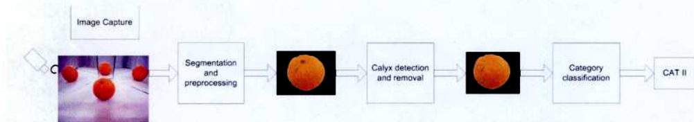
Fig. 4.2: Example of the calyx detection system where an image is analyzed, its calyx is detected and removed, and the orange is classified.
