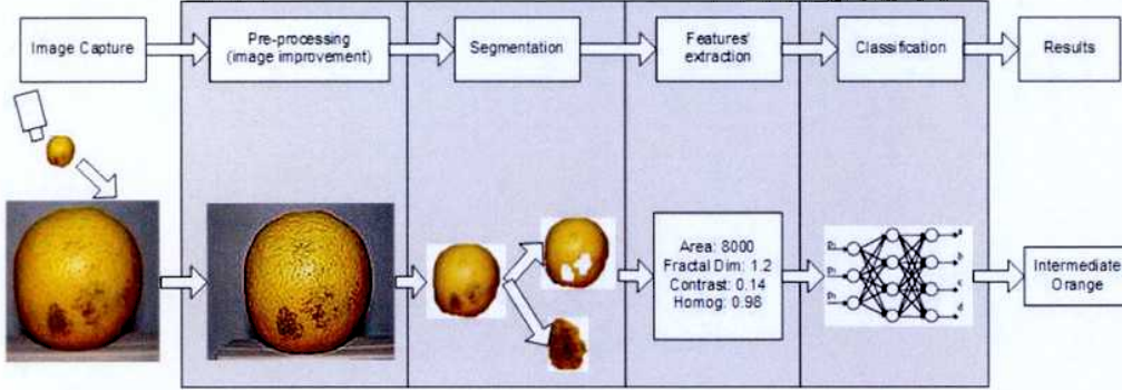
Fig. 5.2: Image processing steps.
