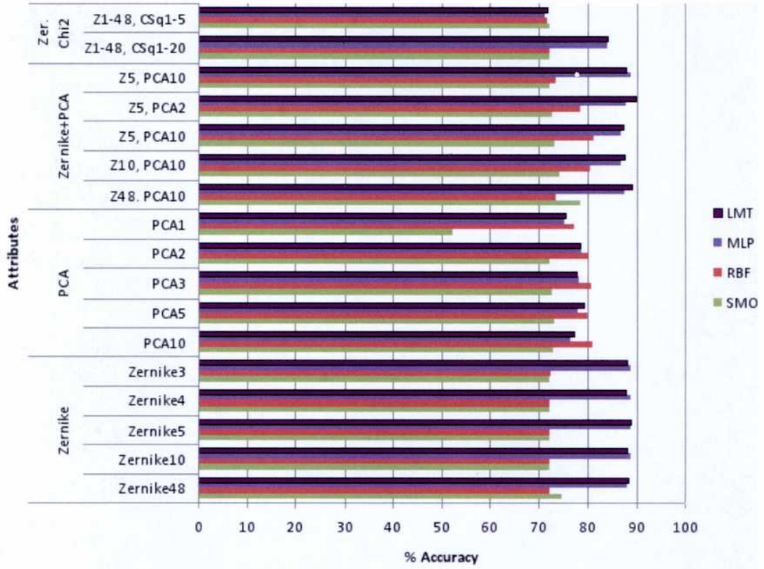
Fig. 4.11: Comparison of classifiers accuracy among the different attributes selection.
