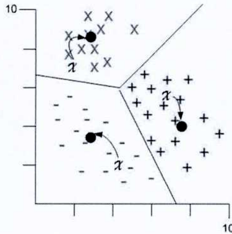
Fig. 2.11: K-Means clustering example: with each iteration, the center of each cluster is moved to the mean position of the group.
