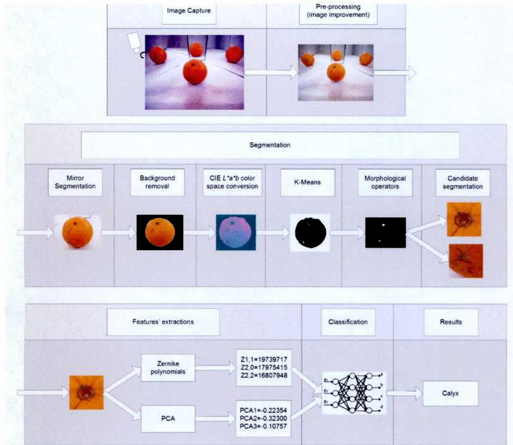
Fig. 4.1: Image processing steps for calyx/defect classification: The oranges images are captured, segmented into subimages of calyx or defect candidates, features are extracted, and the image is classified as calyx or defect.
