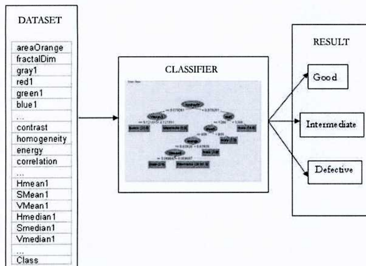
Fig. 5.1: Input-Process-Output diagram of the system where features are extracted, processed and classified
