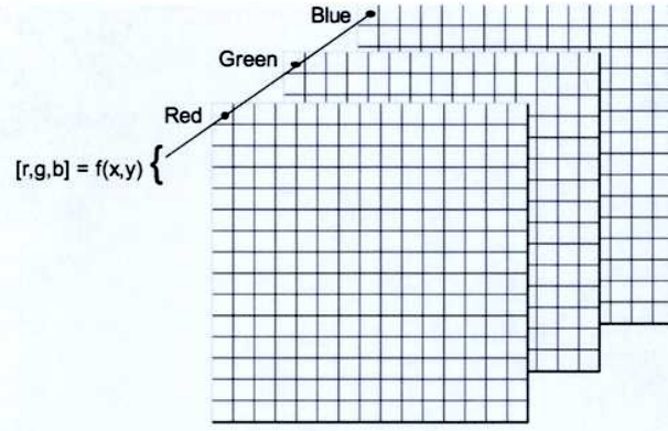
Fig. 2.3: RGB image made of three layers.
