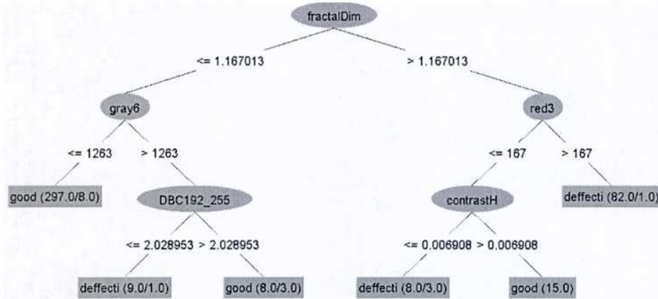
Fig. 5.6: J48 decision tree for only two classes: 'good' and 'defective'.
