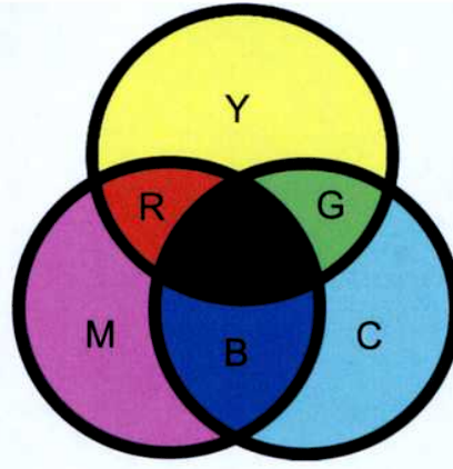
Fig. 2.5: Subtracting Colors of light: Subtracting magenta and cyan from white form blue, subtracting magenta and yellow from white form red, subtracting cyan and yellow from white form green, and subtracting cyan, magenta and yellow form black
