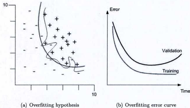
Fig. 2.10: Overfitting example
