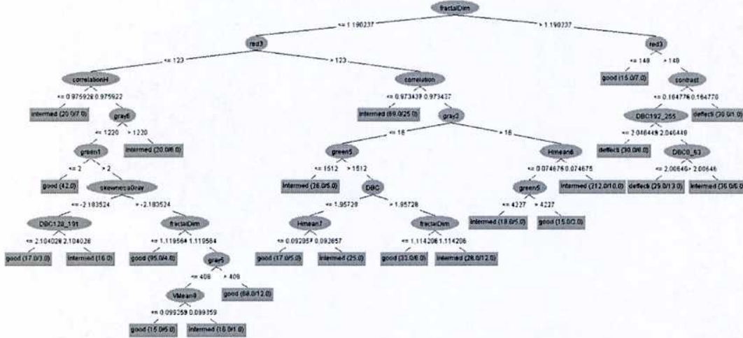
Fig. 5.5: J48 Decision tree
