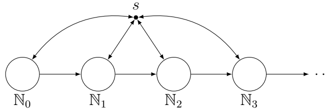
Figure 3.2: The model \mathcal{M} . The transitive connections between the cliques \mathbb{N}_i are not shown.
