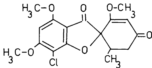
Griseofulvina
