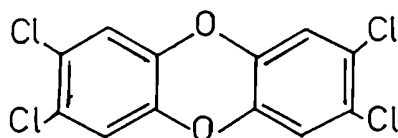
2,3,7,8-tetraclorodibenzo-p-dioxina (TCDD)
