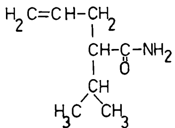
Alilisopropilacetamida (AIA)
