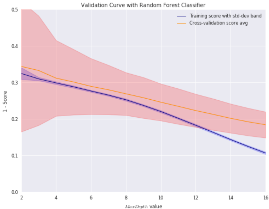
Figure 5.2.1 Validation curve on the tree-depth hyperparameter values for the Random Forest learner. The mean CV scores for the 1 - Accuracy score is shown for a CV run experiment on Problem 2
