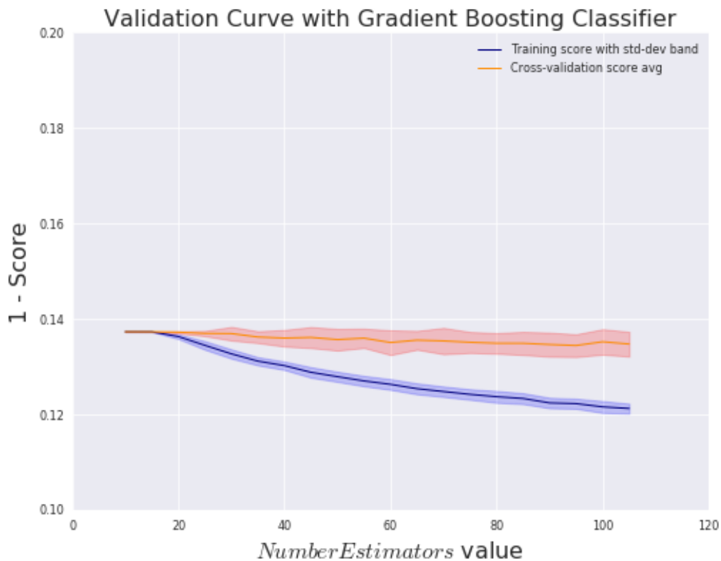
Figure 5.3.2 Validation curve for the number of trees hyperparameter of the Gradient Boosting Tree learner. The mean CV scores for the 1 - Accuracy score is shown for a CV run experiment on Problem 2
