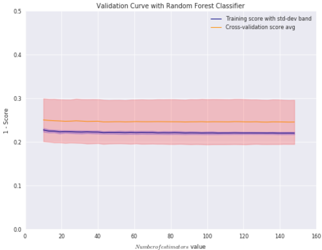
Figure 5.2.2 Validation curve on the number of trees hyperparameter values, for the Random Forest learner. The mean CV scores for the 1 - Accuracy score is shown for a CV run experiment on Problem 2
