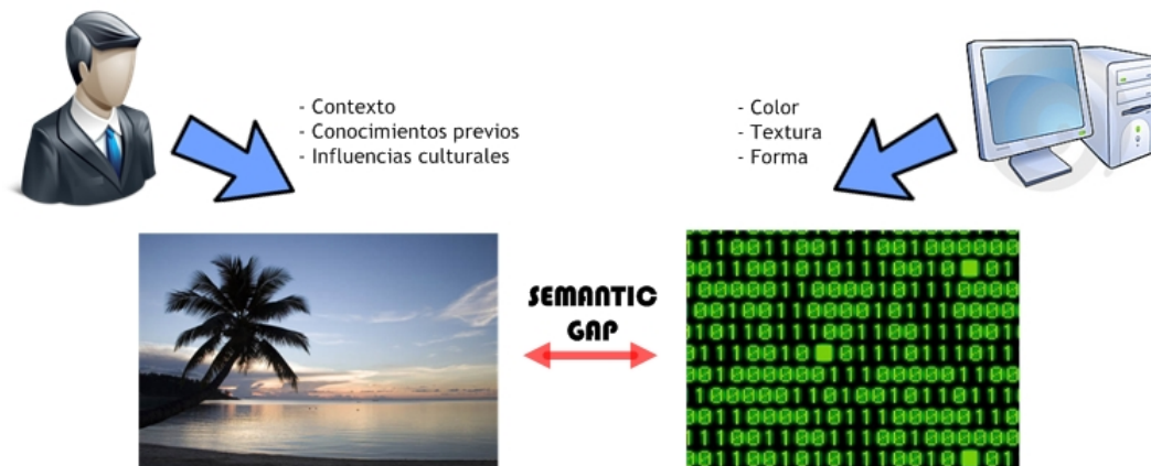
Figura 2.1: Semantic Gap
