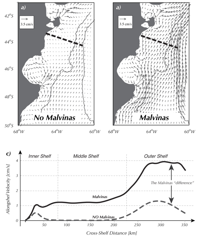
Fig. 9. (a) Depth averaged velocities in EXP2; (b) EXP1; (c) Alongshelf velocities across the section shown in the upper panels. The differences between these two experiments are mainly due to the MC.
