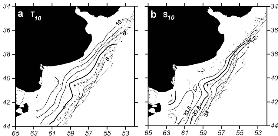
Fig. 7. Temperature (a) and salinity (b) at 10 m depth from hydrographic data collected in July 1996. The heavy contours are 7°C and 33.8, the station locations are indicated (+), station 527 with a bold symbol. The dotted lines represent the 100 and 200 m isobaths from GEBCO.
