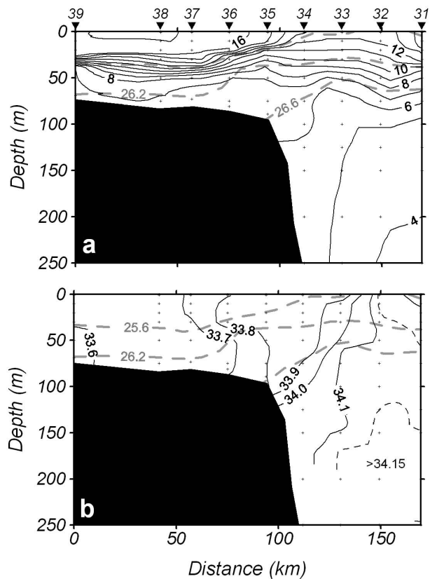
Fig. 2. Temperature (a) and salinity (b) sections across the Patagonia shelf break at 42° S collected in March 1994. The station locations are shown in Fig. 1a. The grey dashed contours are isopycnals ( \sigma_T , \text{kg m}^{-3} ).
