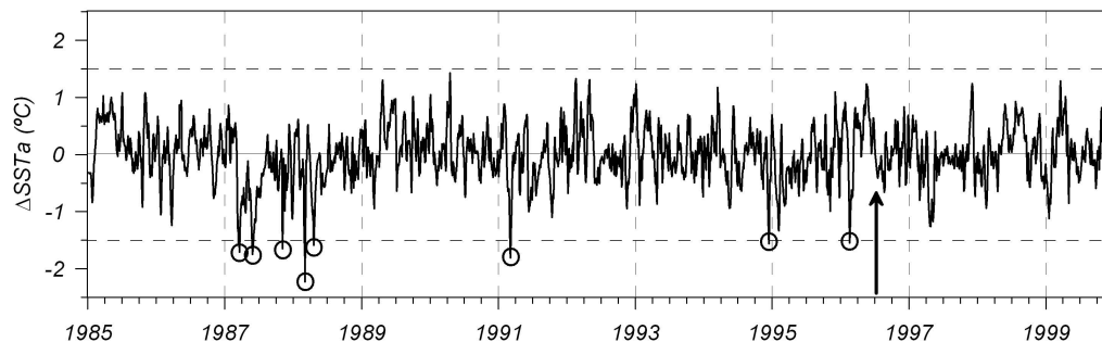
Fig. 6. Time series of difference in SSTa between site A and region III ( \Delta\text{SSTa} ), see Fig. 1 and text. The open circles indicate events where \Delta\text{SSTa} < -1.5 . The heavy arrow indicates the time of occupation of the R/V Holmberg cruise.
