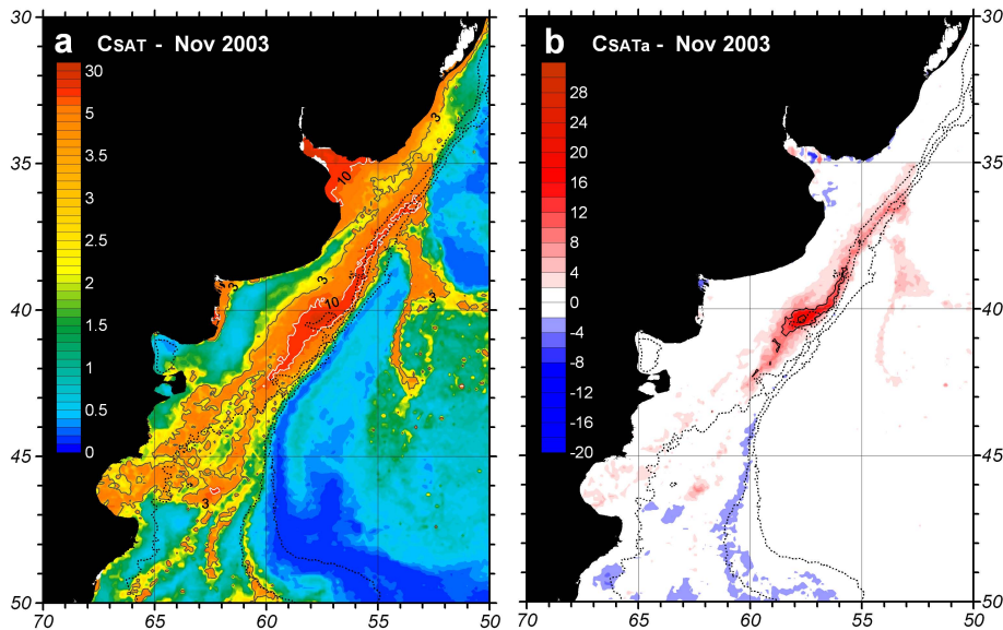
Fig. 11. Mean surface chlorophyll- a distribution (a) and anomaly (b) in November 2003 based on SeaWiFS data. The 3 \text{ mg m}^{-3} (black) and 10 \text{ mg m}^{-3} (white) contours are shown in (a) and the 10 and 20 \text{ mg m}^{-3} in (b). The dotted lines in both panels are the 100, 200 and 1000 m isobaths from GEBCO.
