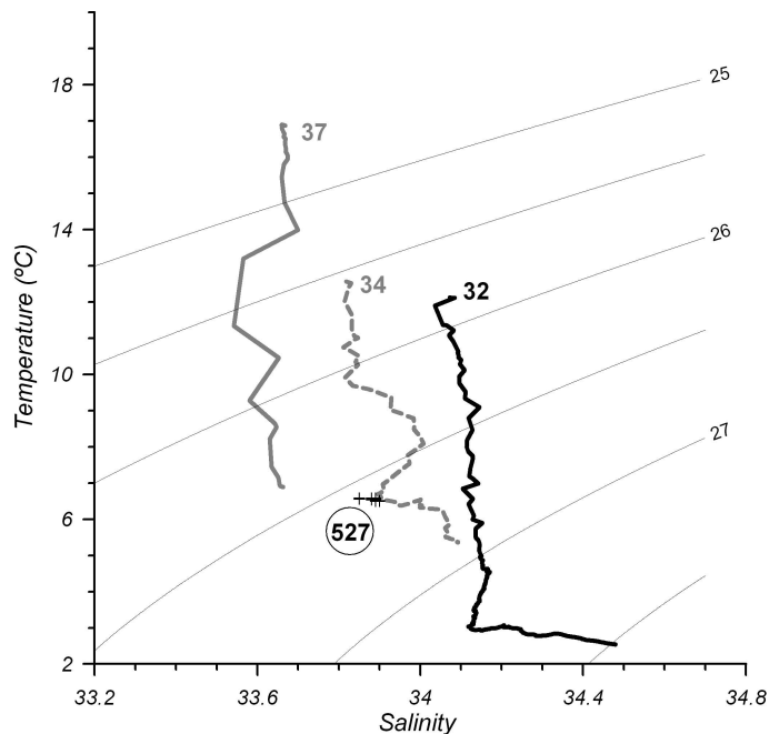
Fig. 3. Temperature-Salinity diagrams of selected stations occupied in the outer shelf (37), shelf break (34) and slope waters (32) in March 1994 (see Fig. 2). Station 527 was occupied in July 1996, 125 km inshore from the 200 m isobath. The thin lines are constant \sigma_T , ( \text{kg m}^{-3} ).
