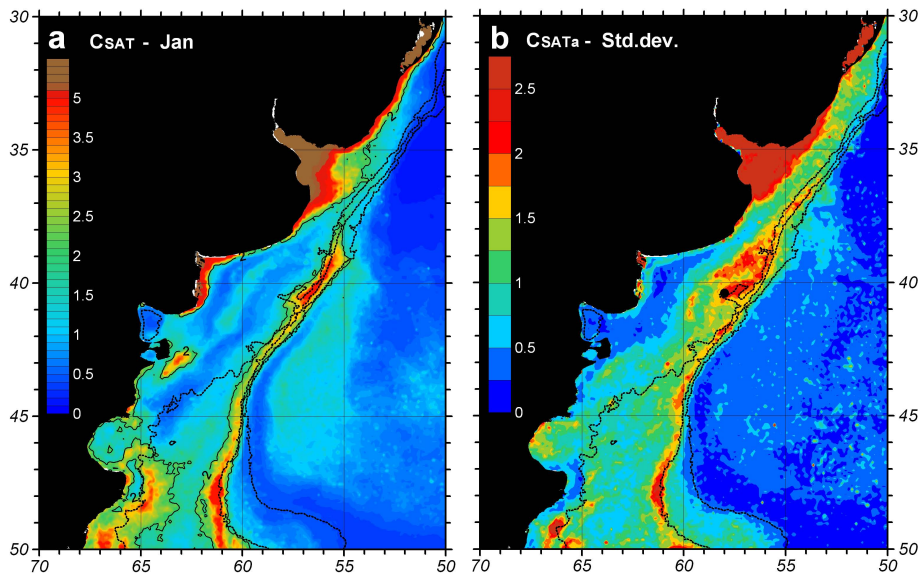
Fig. 9. (a) Mean January surface chlorophyll- a distribution (1998–2007) based on SeaWiFS data (CSAT). The solid line indicates the 2 mg m -3 contour. (b) Standard deviation of the record-length monthly anomalies (CSATa). The black dot in (b) is the position of site A (see Fig. 1). The dotted lines in both panels are the 100, 200 and 1000 m isobaths from GEBCO.
