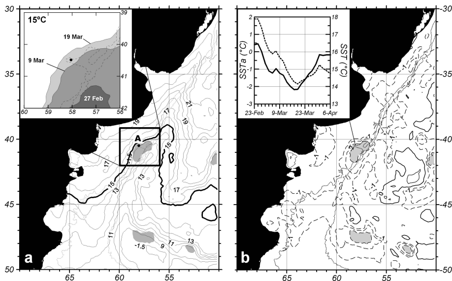
Fig. 4. Satellite derived SST distribution (a) and SST anomalies (b) on 17 March 1986, both in °C. The heavy contour in (a) is the 15°C isotherm and the shaded contours in (b) are anomalies lower than -2^{\circ}\text{C} , also reproduced in (a). The dotted lines in both panels are the 100 and 200 m isobaths from GEBCO. The location of site A (●) is indicated in (a). The inset in (a) shows the evolution of the 15°C isotherm on 27 February, 9 and 19 March 1986, with waters colder than 15°C shaded. The inset in (b) shows the SST (°C, dotted line) and SSTa (°C, heavy line) time series at A (see text).
