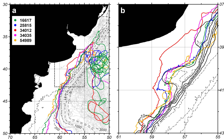
Fig. 10. Trajectories of WOCE surface drifters in the western South Atlantic. (a) All observed drifters in grey, color tracks indicate drifters exhibiting relatively sharp inshore loops near 41° S. (b) Expanded view of the region indicated by the dashed rectangle in (a) with color drifter tracks overlapped with lines of constant potential vorticity (black contours in 10^{-7} \text{ m}^{-1} \text{ s}^{-1} ). The dashed lines in both panels are the 100, 200, 1000, 2000 and 3000 m isobaths from GEBCO.
