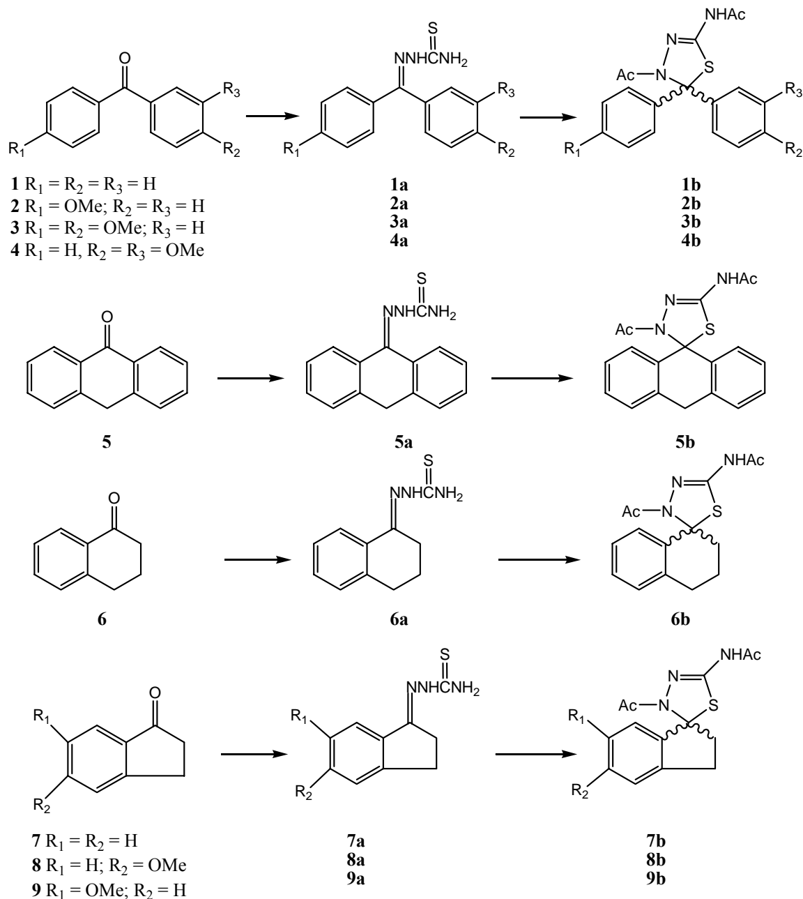
Scheme 1
