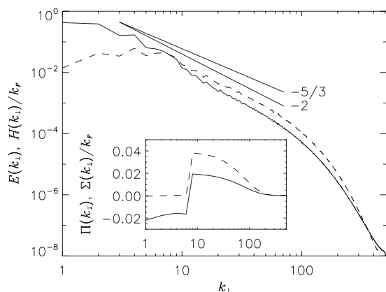
FIG. 10. Perpendicular energy and helicity spectra in run B with Ro=0.06 , with same labels as in Fig. 8. Kolmogorov and k^{-2} scaling laws are shown as a reference. The inset shows the perpendicular energy and helicity fluxes.
