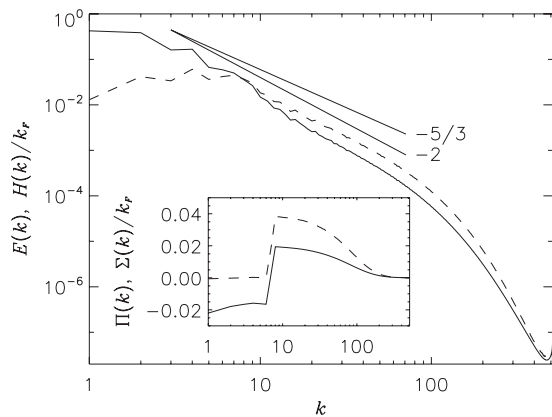
FIG. 9. Isotropic energy and helicity spectra in run B with Ro=0.06 (same labels as in Fig. 8); k^{-5/3} (Kolmogorov), and k^{-2} scaling laws are shown as a reference. The inset gives the isotropic energy and helicity fluxes. Note the excess of (normalized) helicity and of its flux in the small scales.
