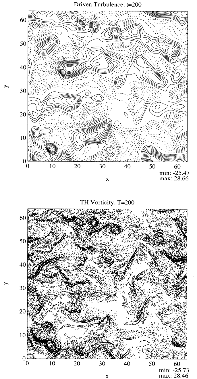
FIG. 16. Driven turbulence simulation (Terry-Horton model). Potential and (generalized) vorticity contour plots at t = 200 , in the stationary state. The lifetime of individual vortices is about ten periods.
