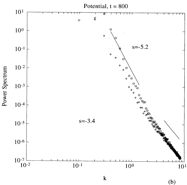
FIG. 13. Power spectrum of the potential at t = 500 and 800 ( W_{k_{x,y}} = \sum_{k_{y,x}} |\phi_{\mathbf{k}}|^2 ). The slopes of the spectrum are indicated at intermediate and large k .
