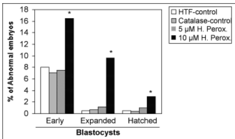
FIGURE 4. Embryo morphology
