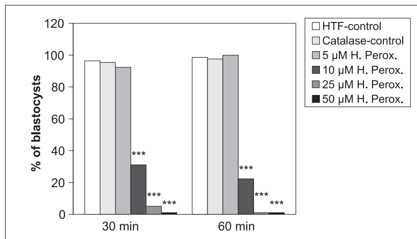
FIGURE 2. Blastocyst development
