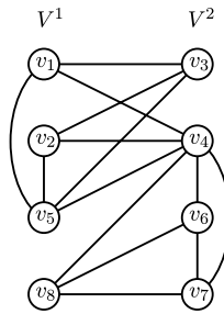
Fig. 1. A graph along with a consistent ordering and 2-partition of the vertices. The non-empty sets N(v_r, j)_< are: N(v_3, 1)_< = \{v_1, v_2\} ; N(v_4, 1)_< = \{v_1, v_2\} ; N(v_5, 1)_< = \{v_1, v_2\} ; N(v_5, 2)_< = \{v_3, v_4\} ; N(v_6, 2)_< = \{v_4\} ; N(v_7, 2)_< = \{v_4, v_6\} ; N(v_8, 2)_< = \{v_4, v_6, v_7\} . Then, \Delta(1)_< = 2 , \Delta(2)_< = 3 .
