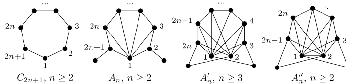
Fig. 3. Some minimal forbidden induced subgraphs for comparability graphs.
