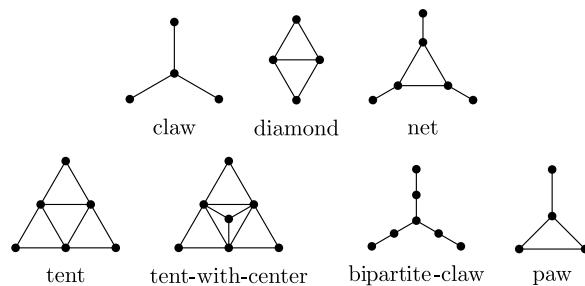
Fig. 1. Some small graphs.
