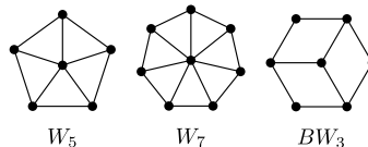
Fig. 2. Graphs W_5 , W_7 and BW_3 .
