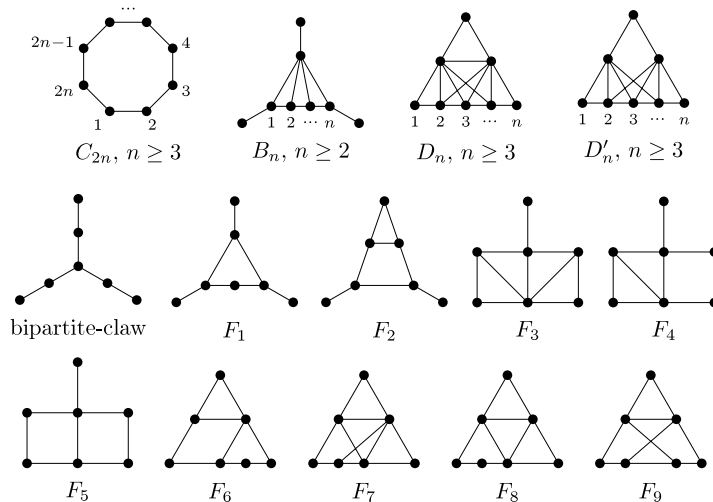
Fig. 4. Some graphs whose complements are minimal forbidden induced subgraphs for comparability graphs.
