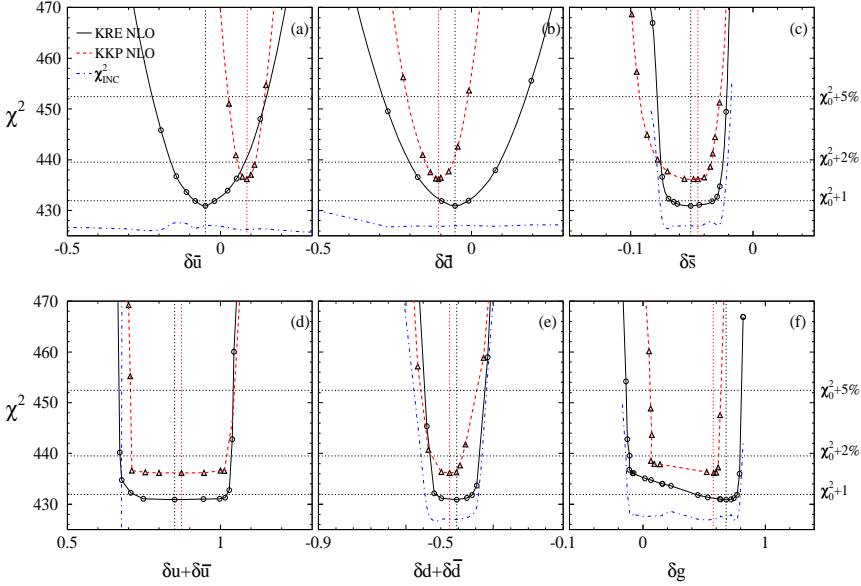
FIGURE 1. \chi^2 profiles for NLO fits obtained using Lagrange multipliers at \hat{Q} = 10 \text{ GeV}^2 .
