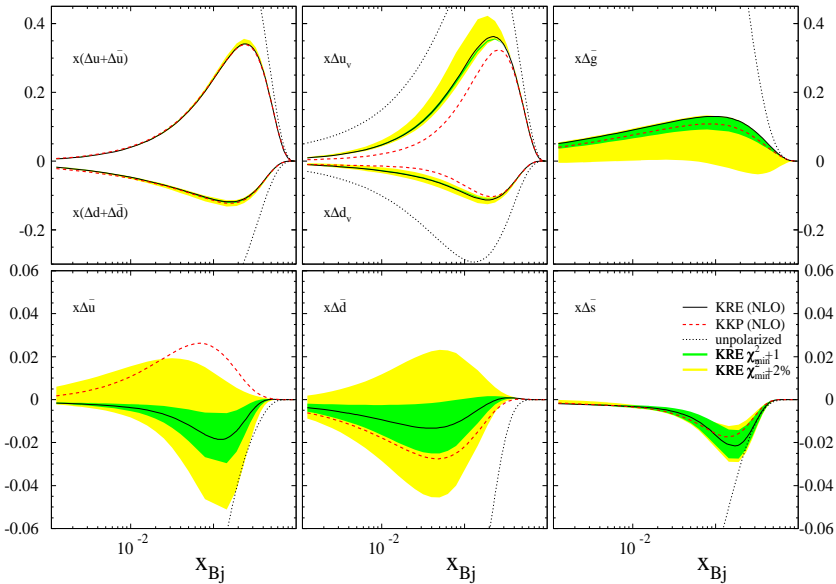
FIGURE 2. Parton densities at Q^2 = 10 \text{ GeV}^2 , and the uncertainty bands corresponding to \Delta\chi^2 = 1 and \Delta\chi^2 = 2\%
