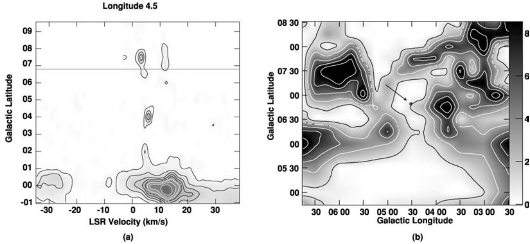
Figure 3. (a) Latitude–velocity map at a longitude of 4^{\circ}5 from the CO Milky Way Survey (e.g. Dame et al. 2001). Contours show T_{\text{A}}^* ranging from 0.3 to 4.5 K in steps of 0.6 K. A line at a constant latitude of 6^{\circ}8 is included to show the location of Kepler’s SNR. The grey-scale goes from 0 to 8.5 K, as shown at the right-hand side of Fig. 3(b). (b) Integrated CO image of the molecular clouds (part of the Ophiuchus complex at 165 pc) in the vicinity of Kepler’s SNR, taken from the Galactic CO data available at http://cfa-www.harvard.edu/mmw/MilkyWayMolClouds.html . The resolution is 8 arcmin and the integration spans over -300 < v < 300 \text{ km s}^{-1} . The contours are at constant T_{\text{A}}^* , ranging from 1 to 9 K in steps of 1 K. The grey-scale is indicated to the right-hand side of the image. An outer radio continuum contour of Kepler’s SNR with location indicated by the arrow.
