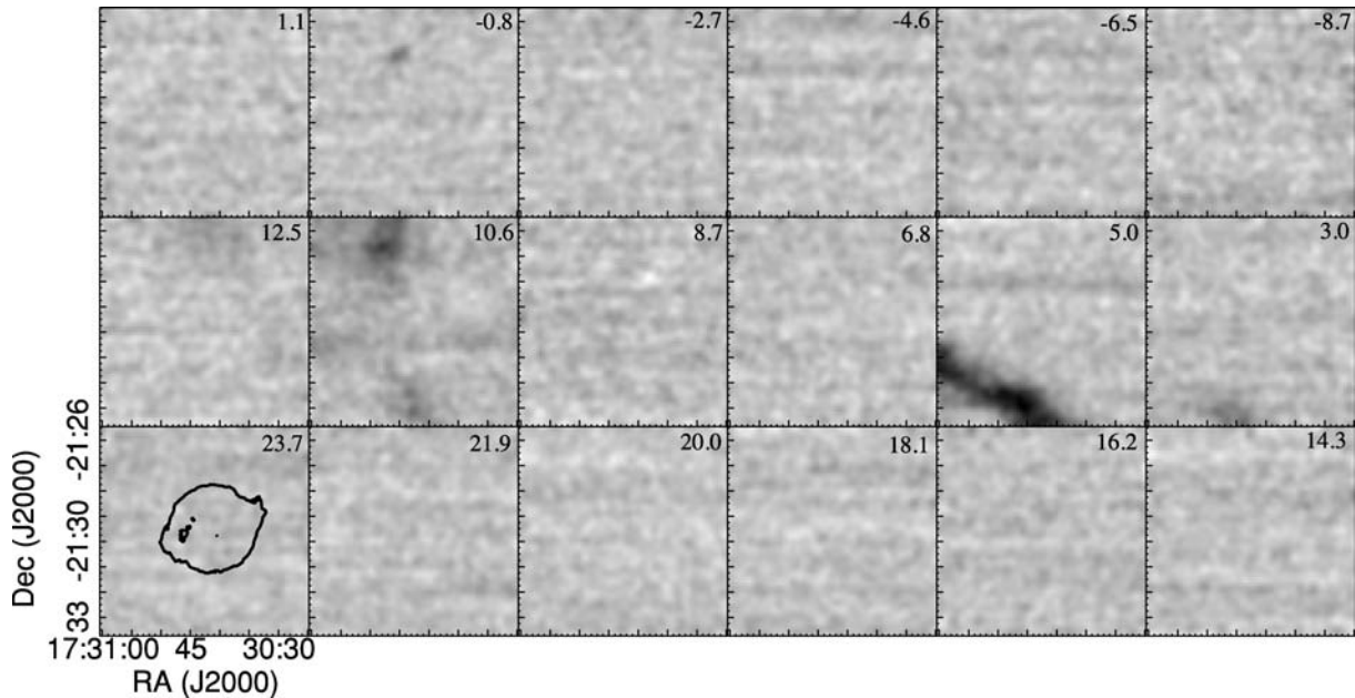
Figure 4. Channel maps of T_{\text{A}}^* across the ^{12}\text{CO}(J=2-1) transition ranging from -10 to 24.6 \text{ km s}^{-1} with velocity width, \Delta v = 1.9 \text{ km s}^{-1} . The images have been smoothed with a 21 arcsec Gaussian. The central velocity is labelled on each grid and the negative grey-scale ranges from -0.41 to 1.2 \text{ K km s}^{-1} . Three clouds are detected: to the south of the remnant at velocities 3-5 \text{ km s}^{-1} ; to the north at velocities 9-11 \text{ km s}^{-1} and a small cloud in the north at velocities 0-2 \text{ km s}^{-1} .
