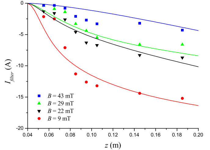
FIG. 5. Current collected by sections of the filter up to the distance z from the cathode, for four different maximum values of the magnetic field. The symbols indicate the experimental values and the lines the theoretical results.
